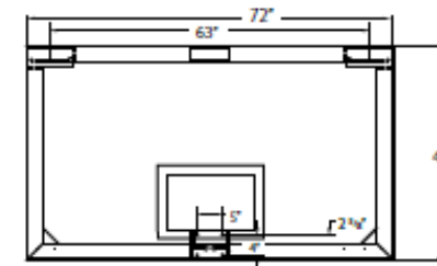
N413-002 Arena® Backboard 72" x 42"
