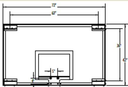
411-007 SuperGlass™ Collegiate® Backboard 72" x 42"
