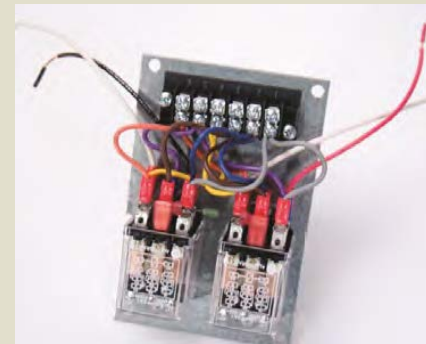
P/N 1037635 Relay board controller
