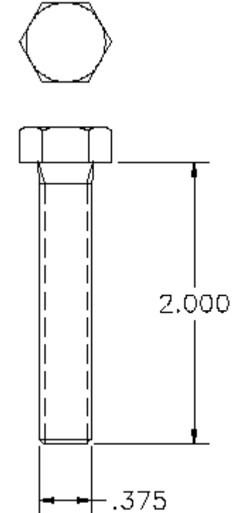
P/N 1000672 MS 3/8 x 2
