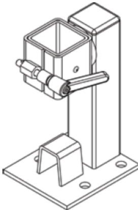
P/N 2067053 Fold down aisle rail socket 9 5/8
