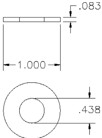
P/N 1000784 3/8 flat washer
