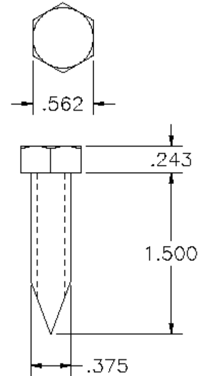
P/N 1000773 Lag Screw 3/8 x 1 1/2
