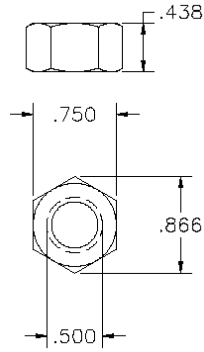
P/N 1000753 1/2 Hex Nut
