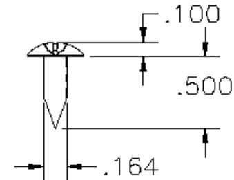
P/N 1000847 Screw #8 x 1/2
