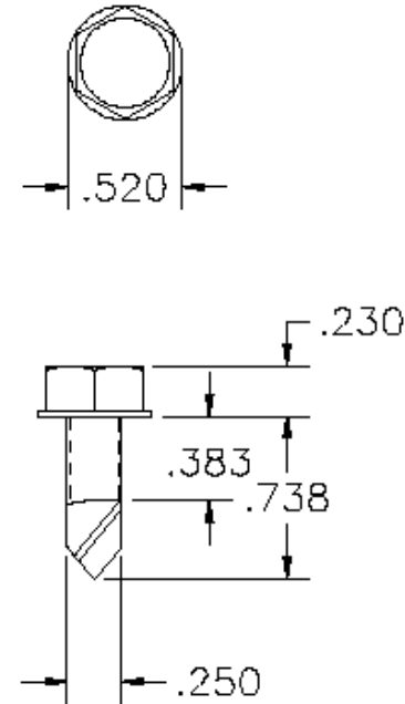
P/N 1000815 Screw 1/4 x 3/4 slfd
