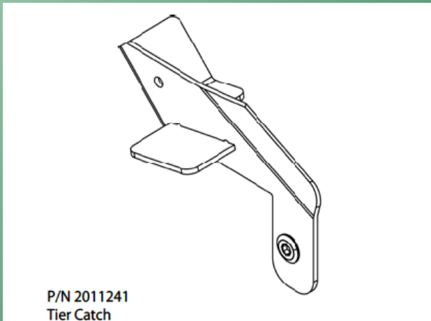
P/N 2011241 Maxam Tier Catch Right
