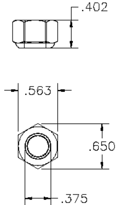
P/N 2022293 3/8 nylon lock Nut
