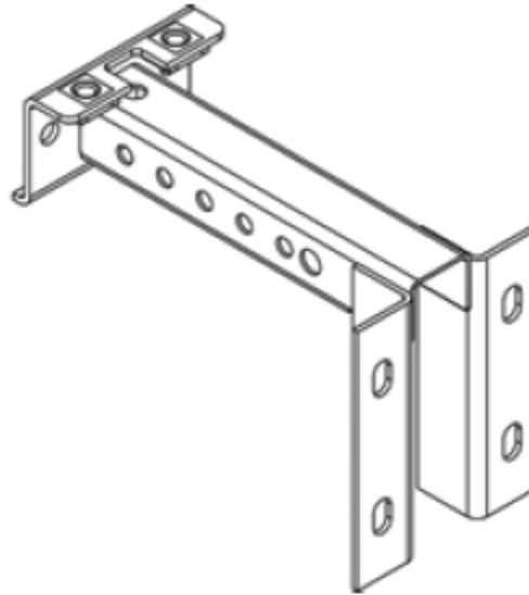
P/N 2010898 Dk stblzr|mxm26 & mxm33|top dk|9.625r & 11.625r
