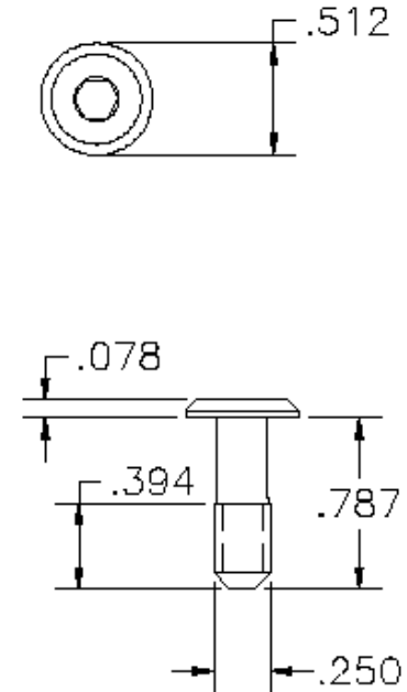
P/N 1012133 Joint connector 1/4 x 13/16 sckt
