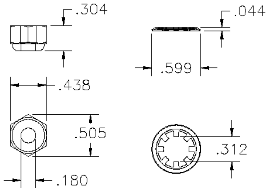
P/N 1000769 12-24 lock nut
