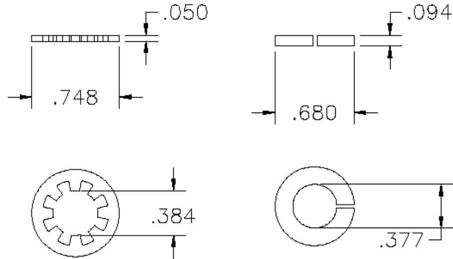
P/N 1000798 3/8 shake proof washer
