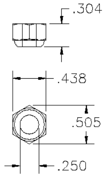
P/N 1000760 1/4 lock Nut
