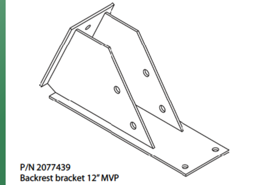
P/N 2077439 Backrest Bracket 12" MVP
