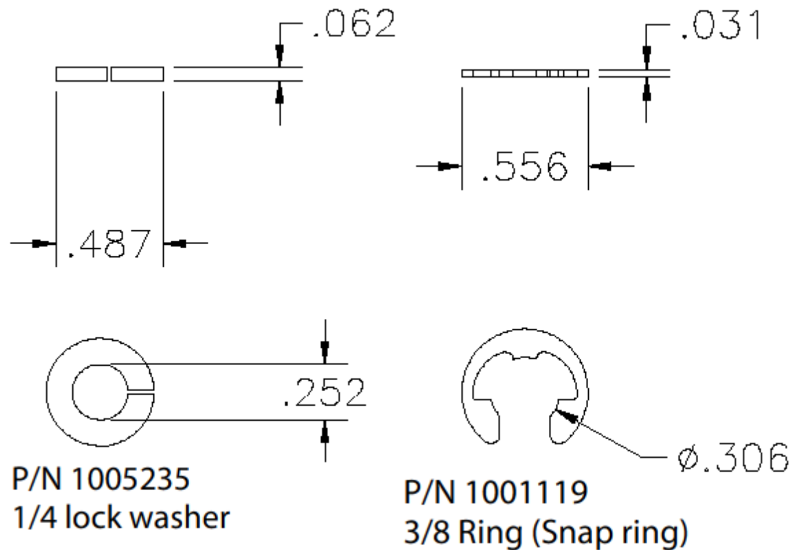
P/N 1005235 1/4 Lock Washer
