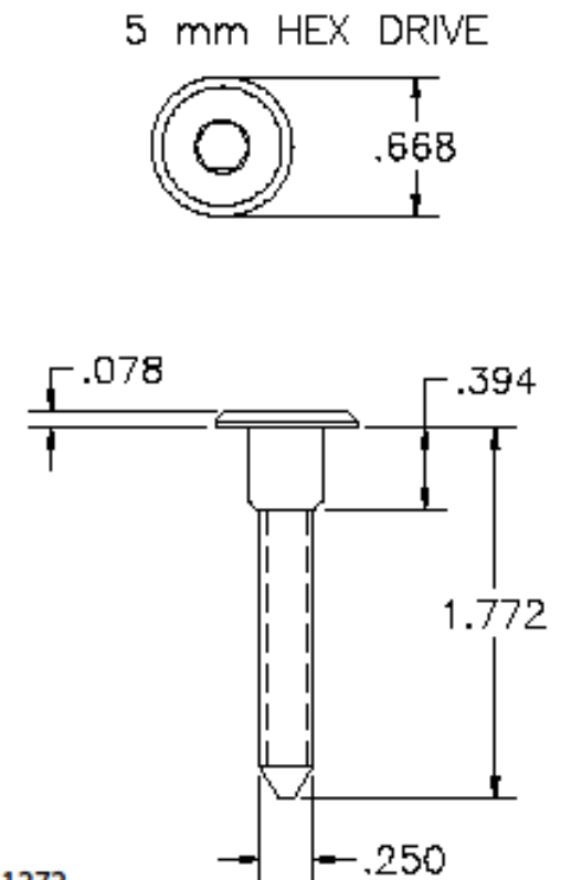
P/N 2011272 Joint Connector 1/4 x 1 3/4
