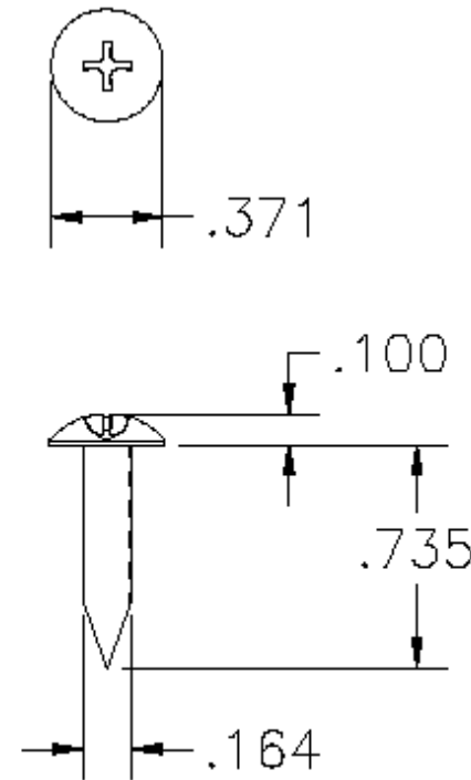
P/N 1042169 Screw #8 x 3/4
