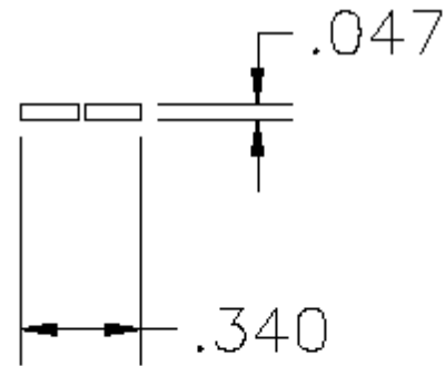
P/N 1038176 3/16 Lock Washer
