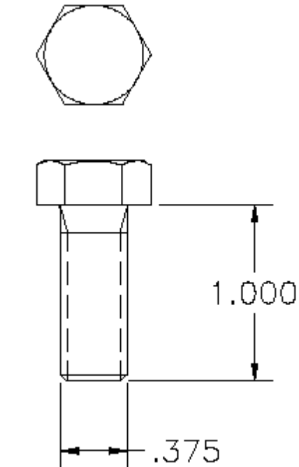
P/N 1000665 MS 3/8 x 1
