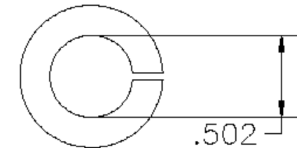
P/N 1000786 1/2 lock washer
