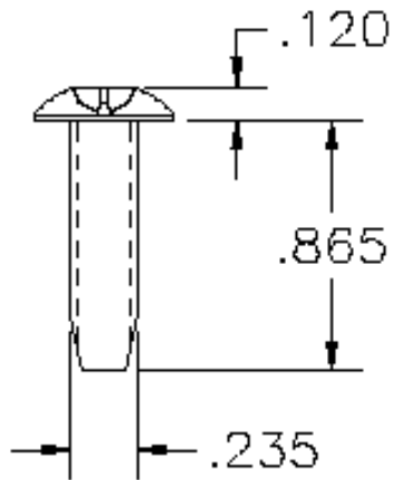
P/N 1016223 Screw 1/4 x 3/4
