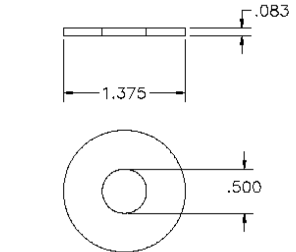
P/N 1000789 1/2 flat washer, 1/8 thk
