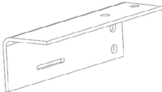
P/N 1002369 Limit switch bracket (close)
