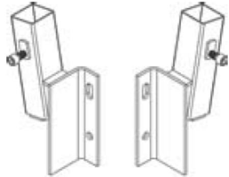
P/N 2024212 RH - 2024213 LH Top Deck Rear End Rail Socket
