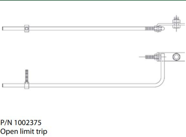
P/N 1002375 Open Limit Trip
