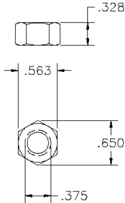
P/N 1000746 3/8 Hex Nut
