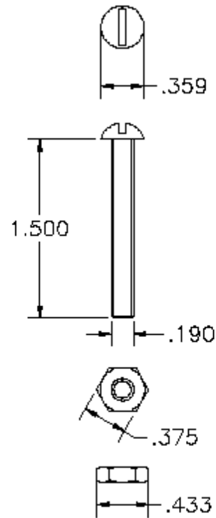
P/N 1000702 Stove bolt 3/16 X 1 1/2
