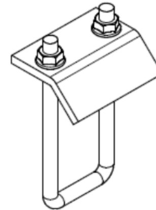
101173821 Double Strut Beam Clamp
