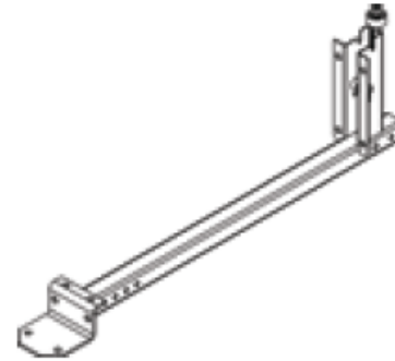
P/N 2016984 Socket supt maxam26 @ stab 9.625
