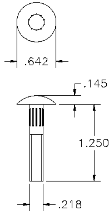
P/N 1001102 12-24 X 1 1/4 step bolt
