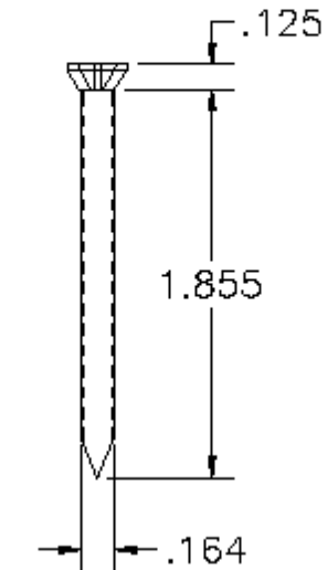
P/N 2035052 Screw #8 x 2, phil fl hd
