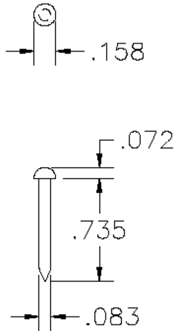
P/N 1001086 Small brads
