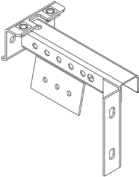
P/N 2011147 RH - 2011152 LH Attchmnt|mxm26 & mxm33| wll|tp frm|9.625r & 11.625r|rh
