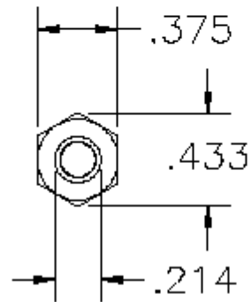
P/N 1036434 #10 hex nut
