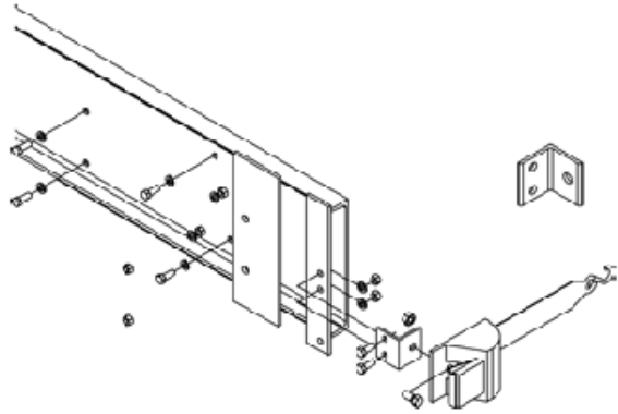
P/N 2070109 Ratchet Strap
