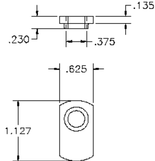
P/N 2077817 3/8 "T" weld Nut
