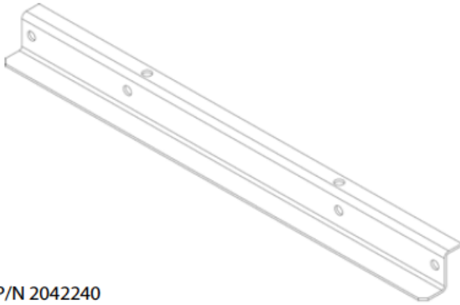
P/N 2042240 Ingot Bracket
