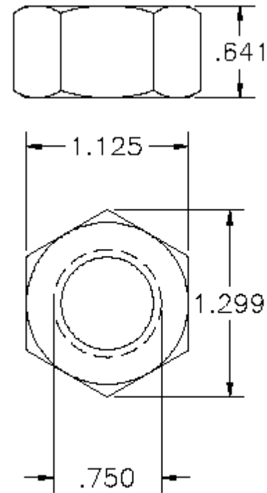
P/N 1000759 3/4 Hex Nut
