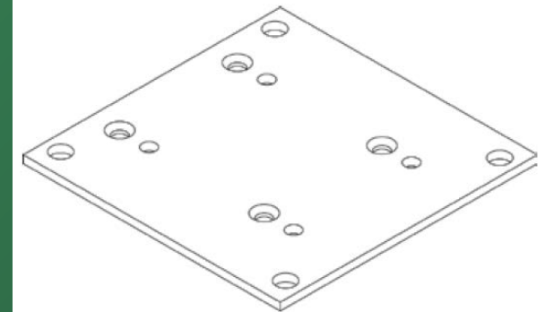
P/N 1027668 Adapter plate
