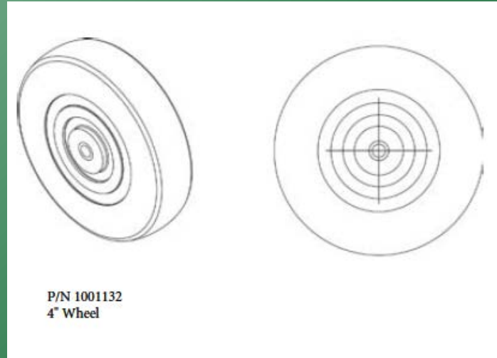
P/N 1005185 - 3" Wheel P/N 1001132 - 4" Wheel P/N 2011007 - 5" Wheel P/N 1020010 - 6" Wheel
