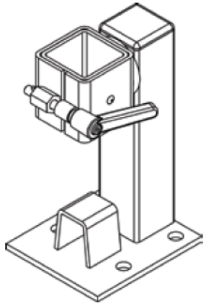
P/N 2067054 Fold down aisle rail socket 11.625
