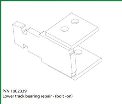
P/N 1002339 Lower Track Bearing Repair
