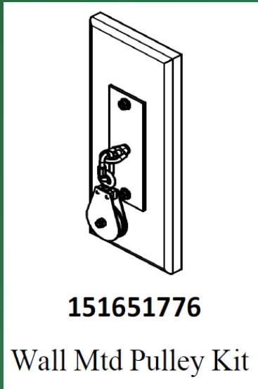
P/N PSS151651776 Wall Mounted Pulley Kit
