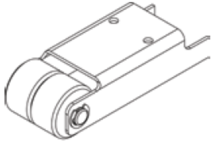
P/N 2033768 Support / 2t / 11.625r
