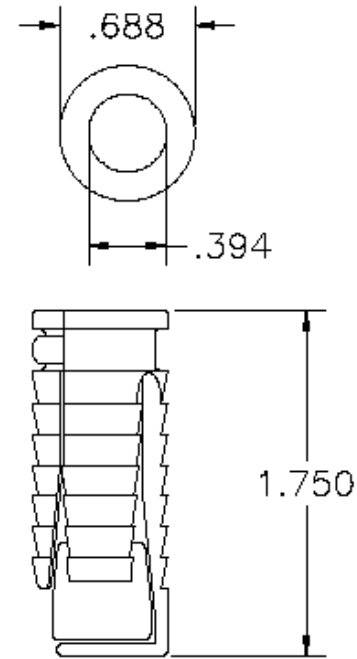
P/N 1007346 Anchor|3/8 exp shld|4way
