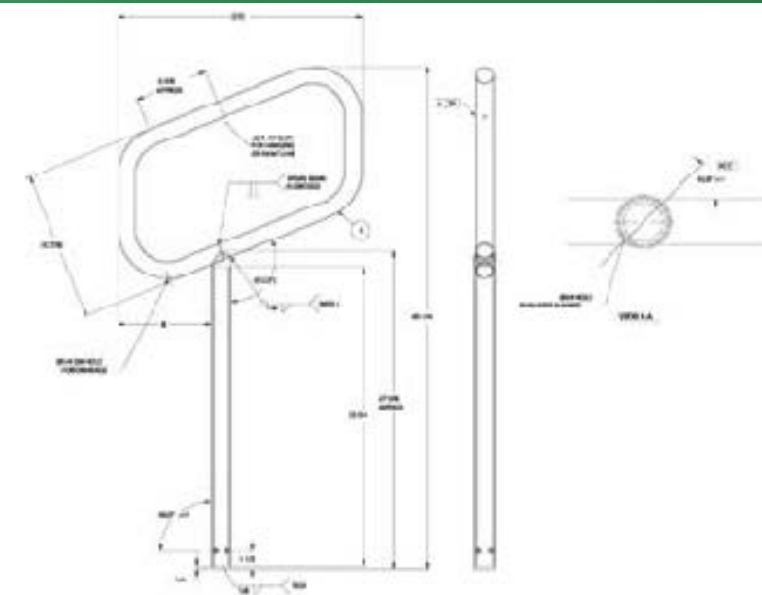
P/N 2102273 P-Rail ( RO26 )
