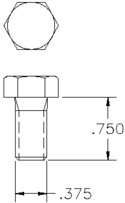
P/N 1000663 MS 3/8 x 3/4
