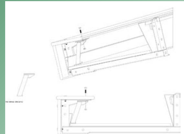
P/N 1005964 Seat Support Repair
