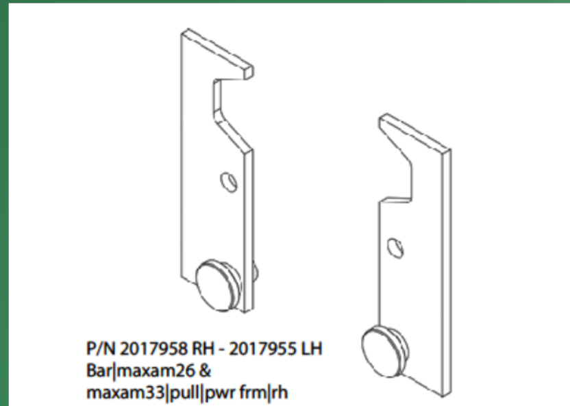
P/N 2017958 - Right P/N 2017955 - Left Power Front Bar
