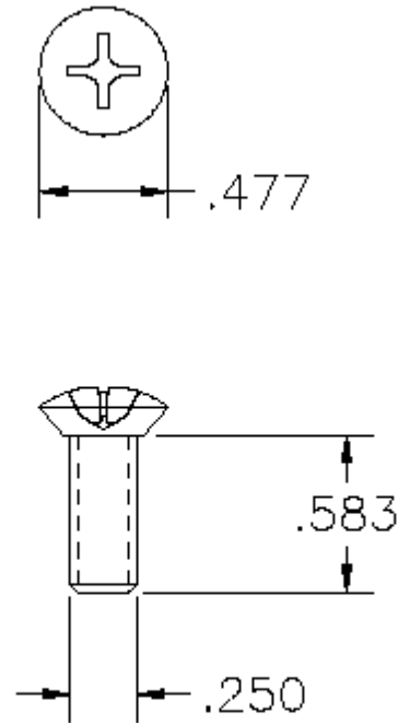
P/N 1000816 MS 1/4 X 3/4
