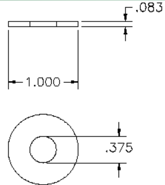
P/N 1035688 3/8 flat Washer, 1/8" thk
