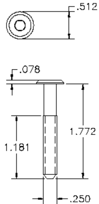
P/N 1022946 Joint connector 1/4 x 1 3/4
