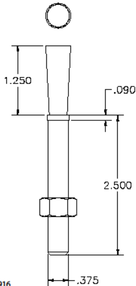
P/N 2018916 Anchor 3/8x 3 3/4
