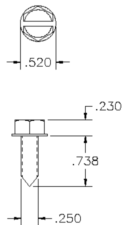
P/N 1000821 Screw #14 x 3/4
