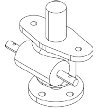
P/N 2042167 Jack screw 1ton 2.250 stroke
