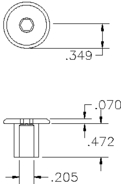
P/N 1015132 1/4 joint connector nut
