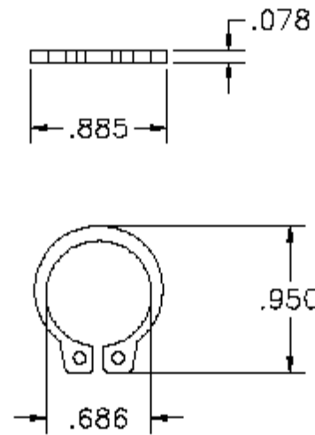
P/N 1042325 Retaining ring 3/4
